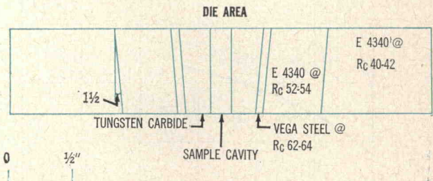
FIGURE 4: Ultra-high-pressure apparatus used by Kennedy and LaMori at UCLA. Pressure in the carbide core is generated by advancing pistons made of GE 883 and 999 tungsten carbide. The pistons are ground to a fit of better than 0.0003 in. to lapped bores in the core.
