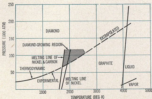
CARBON phase diagram showing theoretical and actual diamond-growing areas, as given by Bovenkerk et al.
